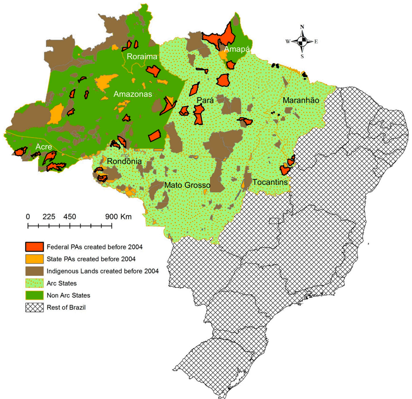
Fig. 1. PAs created before 2004 in Brazil's Legal Amazon region.
